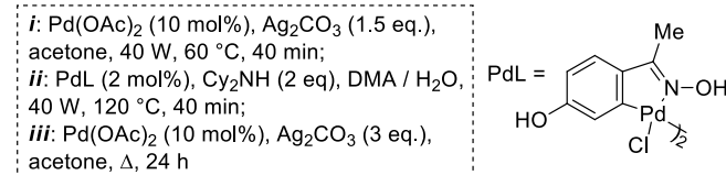
Scheme 20. Synthesis of pterocarpan 15 , 89–90 .
