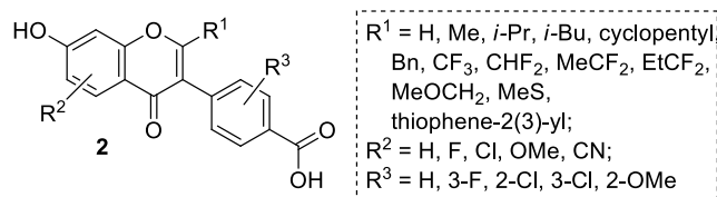
Figure 2. 4-(7-Hydroxy-4-oxo-4 H -chromen-3-yl)benzoic acids 2 – inhibitors of S -nitrosoglutathione reductase.
