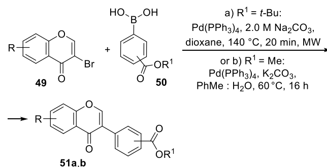
Scheme 12. Synthesis of isoflavones 51a,b – precursors for antagonists of the bradykinin B1 receptor.
