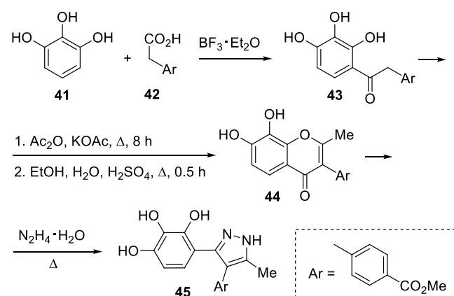
Scheme 9. Synthesis of isoflavone 44 – a precursor of inhibitors of glycogen synthase.
