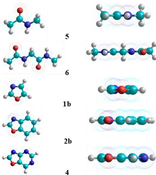
Figure 1. Optimized geometry of the compounds 1b , 2b , 4-6 .
