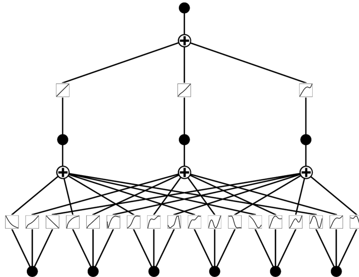
Fig. 3. Network architecture KAN_6_3_1_grid3_k5
