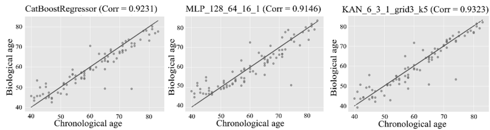
Fig. 2. Correlation graphs of models with the best accuracy rates
